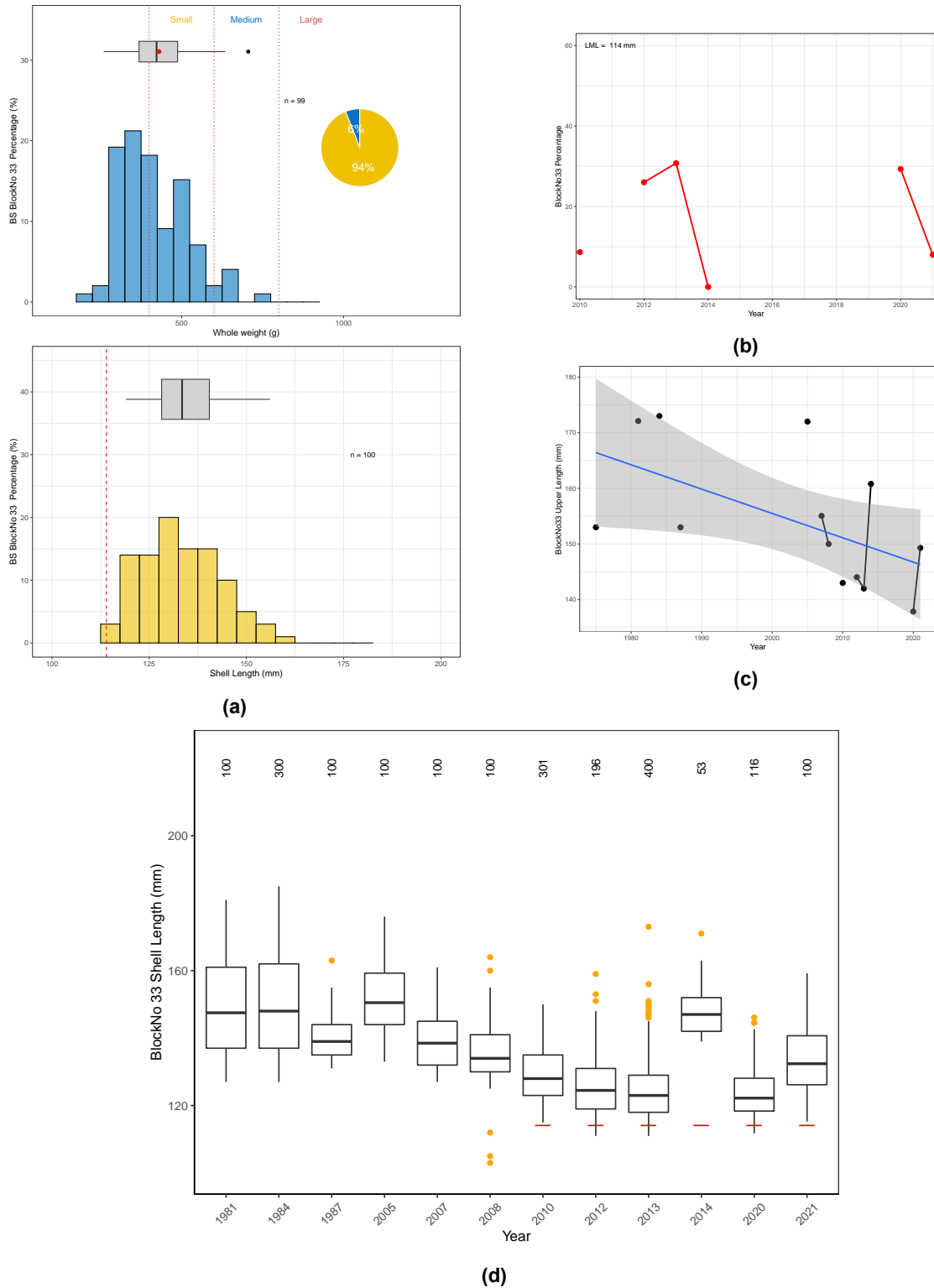
Figure 3.88: Block 33 BSZ: a) Weight (top) and length (bottom) frequency distributions recorded at processing factories in 2021. Horizontal box plots represent summary weight and length distributions. Pie plot represents percentage composition of weight gradings (vertical dashed red lines) for abalone weighed; b) proportion of commercial catch within 5 mm of current legal minimum length (LML). Note: Dashed red line are catch proportions prior to LML change (vertical dashed red line) within 5 mm of current LML; c) Upper 5th percentile of shell length frequency distributions; d) Boxplot of length frequency distributions between 1984 and 2021. Red line under each boxplot indicates LML for that year. Note: Red vertical dashed line represents a pause in sampling of more than one year prior to 2021. Number of abalone measured given above each boxplot.
