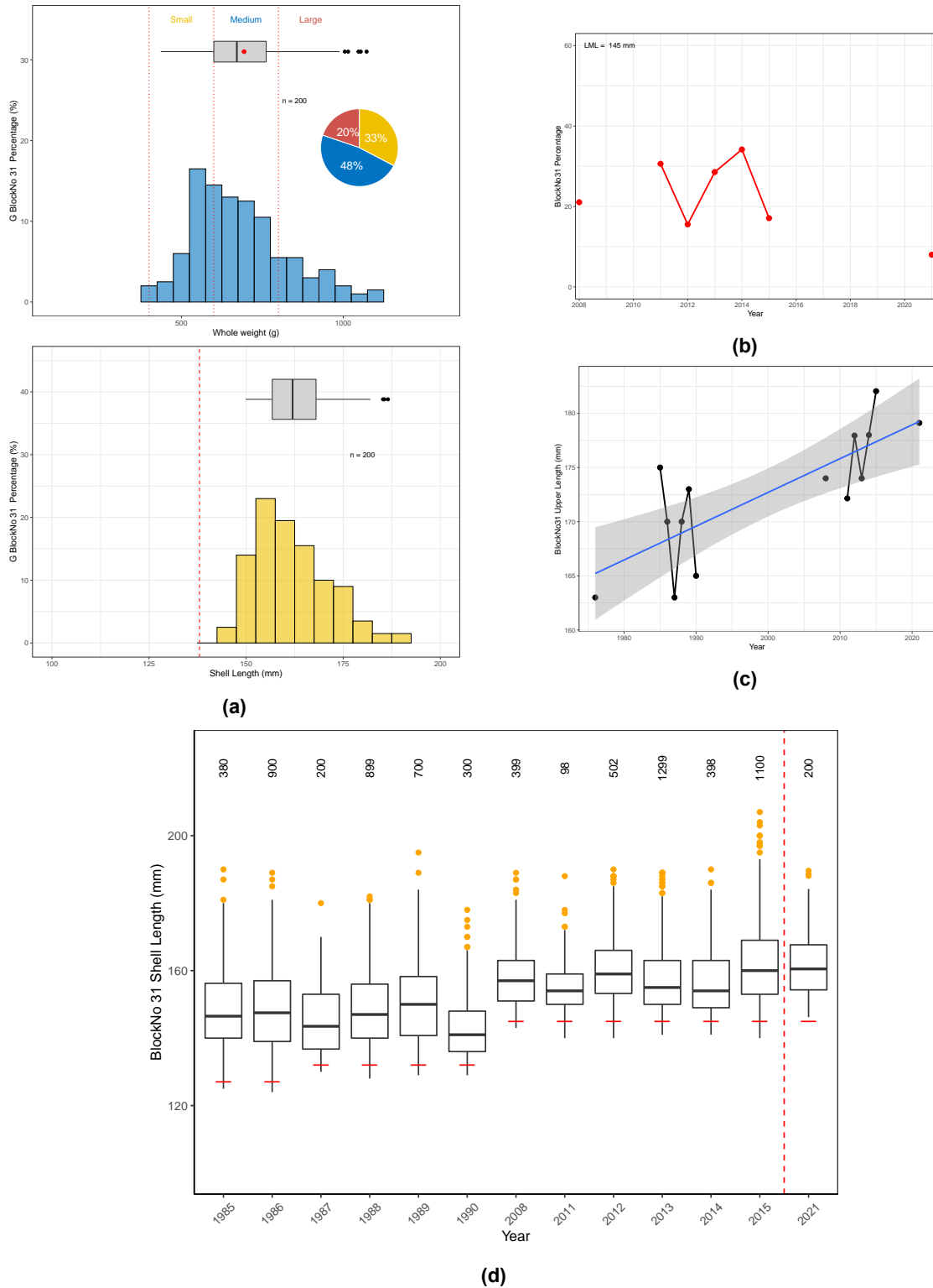
Figure 3.91: Block 31 GZ: a) Weight (top) and length (bottom) frequency distributions recorded at processing factories in 2021. Horizontal box plots represent summary weight and length distributions. Pie plot represents percentage composition of weight gradings (vertical dashed red lines) for abalone weighed; b) proportion of commercial catch within 5 mm of current legal minimum length (LML). Note: Dashed red line are catch proportions prior to LML change (vertical dashed red line) within 5 mm of current LML; c) Upper 5th percentile of shell length frequency distributions; d) Boxplot of length frequency distributions between 1984 and 2021. Red line under each boxplot indicates LML for that year. Note: Red vertical dashed line represents a pause in sampling of more than one year prior to 2021. Number of abalone measured given above each boxplot.
