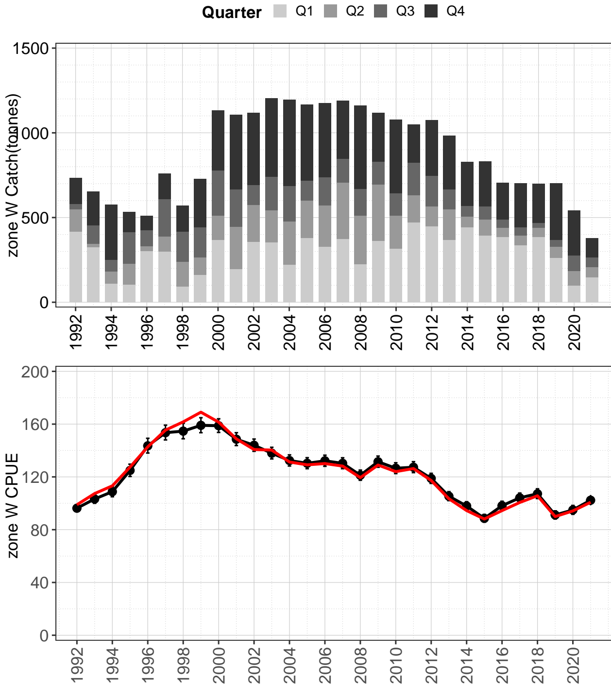
Figure 3.20: Zone-wide catch and catch rate for Western Zone blacklip abalone, 1992–2021. Upper plot: catch (t) by quarter pooled across blocks currently classified as Western Zone. Lower Plot: standardised CPUE (black line) and geometric mean CPUE (red line).
