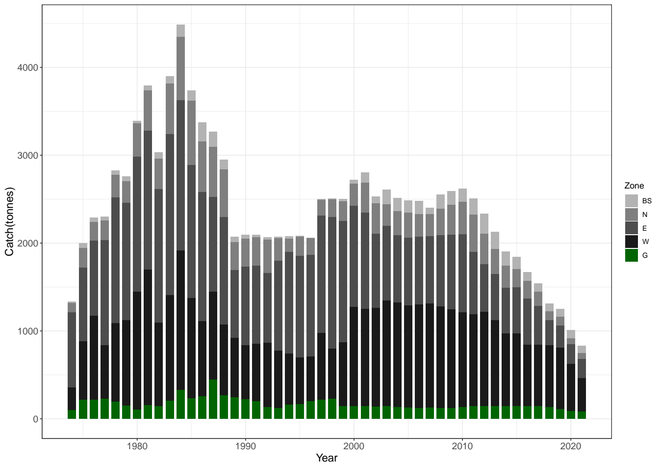
Figure 1.1: Annual blacklip abalone ( Haliotis rubra ) and greenlip abalone ( H. laevigata ) from 1974 to 2021. Bars colour coded by current zonation system.
