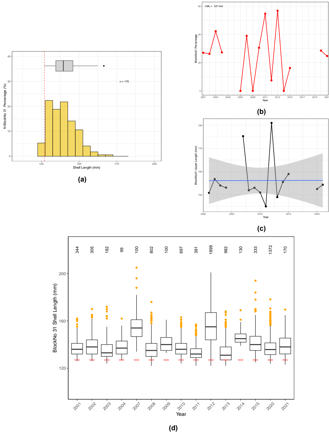
Figure 3.86: Block 31 NZ: a) Length frequency distribution recorded by diver-based measuring board in 2021. Horizontal box plots represent summary length distribution. Vertical dashed red line represents LML; b) Proportion of commercial catch within 5 mm of current legal minimum length (LML); c) Upper 5th percentile of shell length frequency distributions; d) Boxplot of length frequency distributions between 1984 and 2021. Red line under each boxplot indicates LML for that year. Note: Red vertical dashed line represents a pause in sampling of more than one year prior to 2021. Number of abalone measured given above each boxplot.
