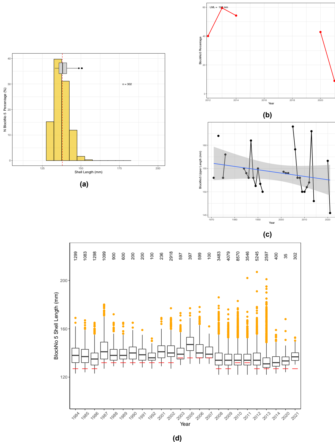
Figure 3.85: Block 5 NZ: a) Length frequency distribution recorded by diver-based measuring board in 2021. Horizontal box plots represent summary length distribution. Vertical dashed red line represents LML; b) Proportion of commercial catch within 5 mm of current legal minimum length (LML); c) Upper 5th percentile of shell length frequency distributions; d) Boxplot of length frequency distributions between 1984 and 2021. Red line under each boxplot indicates LML for that year. Note: Red vertical dashed line represents a pause in sampling of more than one year prior to 2021. Number of abalone measured given above each boxplot.
