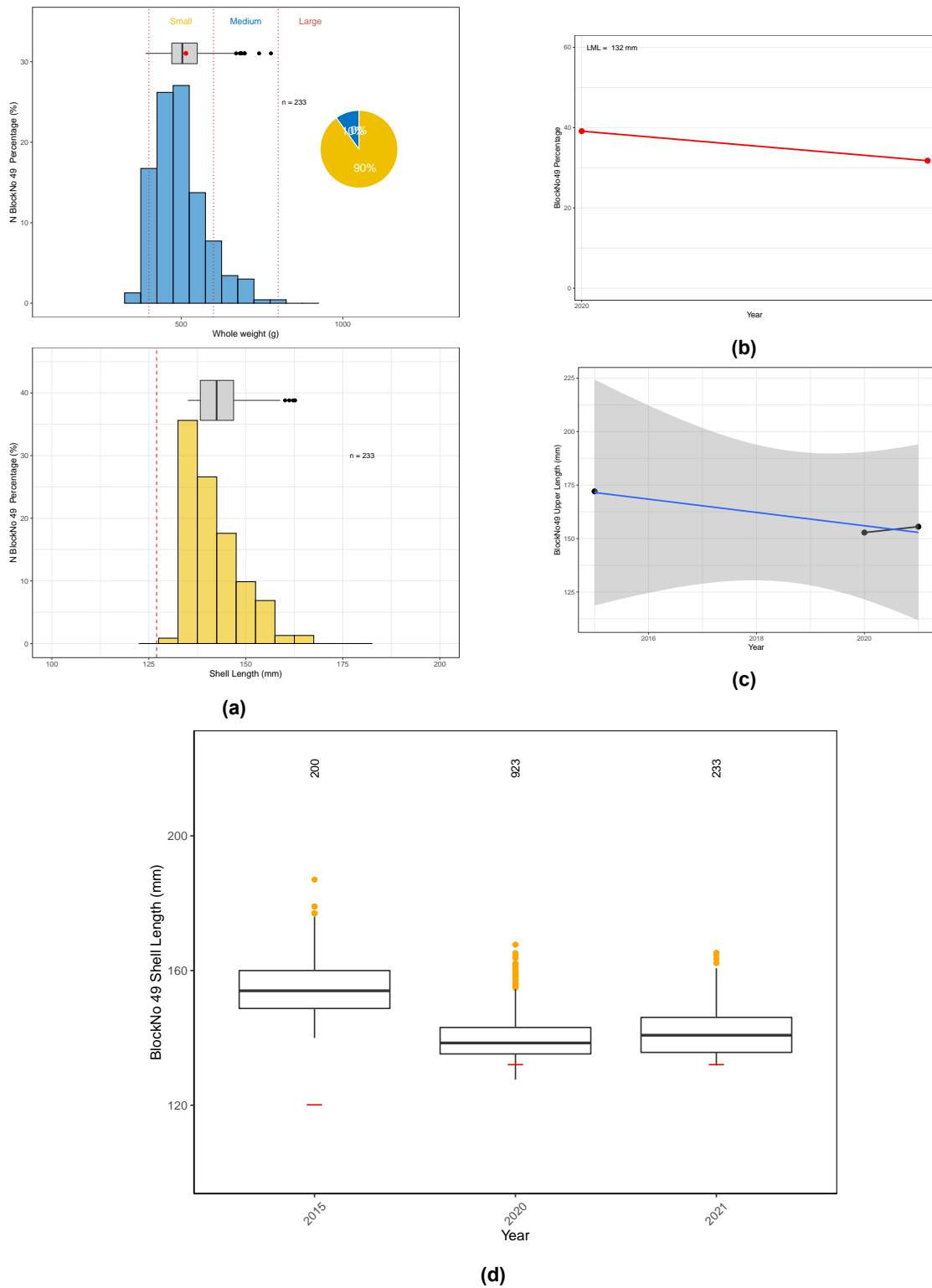
Figure 3.87: Block 49 NZ: a) Weight (top) and length (bottom) frequency distributions recorded at processing factories in 2021. Horizontal box plots represent summary weight and length distributions. Pie plot represents percentage composition of weight gradings (vertical dashed red lines) for abalone weighed; b) proportion of commercial catch within 5 mm of current legal minimum length (LML). Note: Dashed red line are catch proportions prior to LML change (vertical dashed red line) within 5 mm of current LML; c) Upper 5th percentile of shell length frequency distributions; d) Boxplot of length frequency distributions between 1984 and 2021. Red line under each boxplot indicates LML for that year. Note: Red vertical dashed line represents a pause in sampling of more than one year prior to 2021. Number of abalone measured given above each boxplot.
