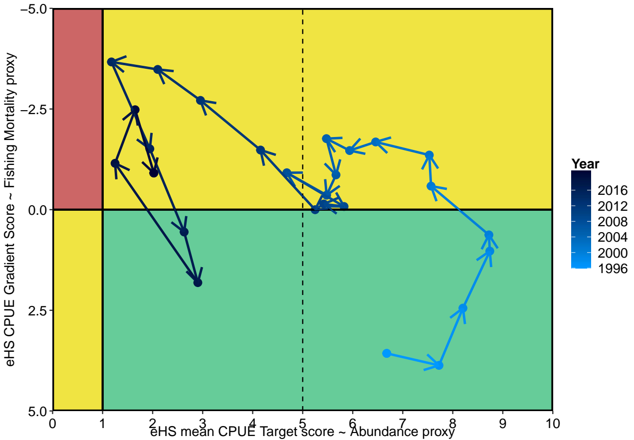
Figure 3.23: Phase plot of fishing mortality and abundance proxies for Western Zone blacklip abalone, 1996–2021. The Gradient 4 PM (y-axis) is used as a proxy for fishing mortality, and the Target CPUE PM is used as a proxy for abundance. Zone score is calculated as a catch-weighted mean of individual block scores.
