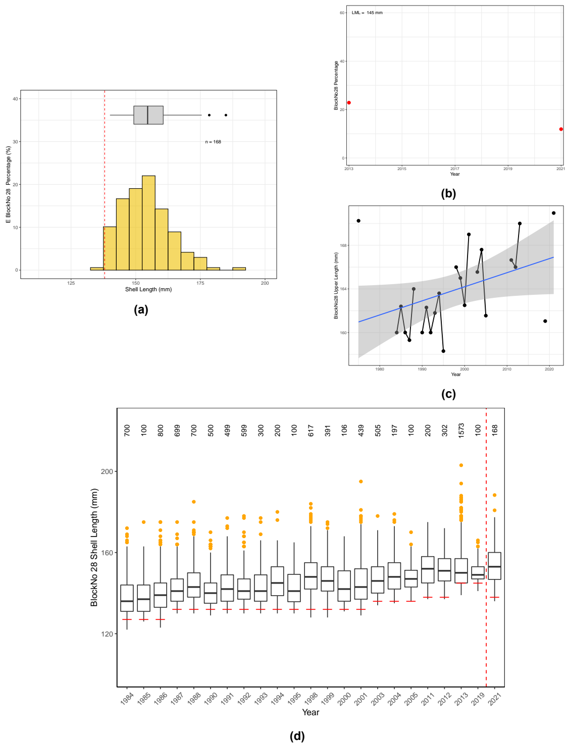
Figure 3.77: Block 28 EZ: a) Length frequency distribution recorded by diver-based measuring board in 2021. Horizontal box plots represent summary length distribution. Vertical dashed red line represents LML; b) Proportion of commercial catch within 5 mm of current legal minimum length (LML); c) Upper 5th percentile of shell length frequency distributions; d) Boxplot of length frequency distributions between 1984 and 2021. Red line under each boxplot indicates LML for that year. Note: Red vertical dashed line represents a pause in sampling of more than one year prior to 2021. Number of abalone measured given above each boxplot.
