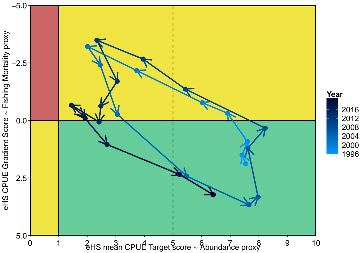
Figure 3.4: Phase plot of fishing mortality and abundance proxies for Eastern Zone blacklip abalone, 1996–2021. The Gradient 4 PM (y-axis) is used as a proxy for fishing mortality, and the Target CPUE PM is used as a proxy for abundance. Zone score is calculated as a catch-weighted mean of individual block scores.
