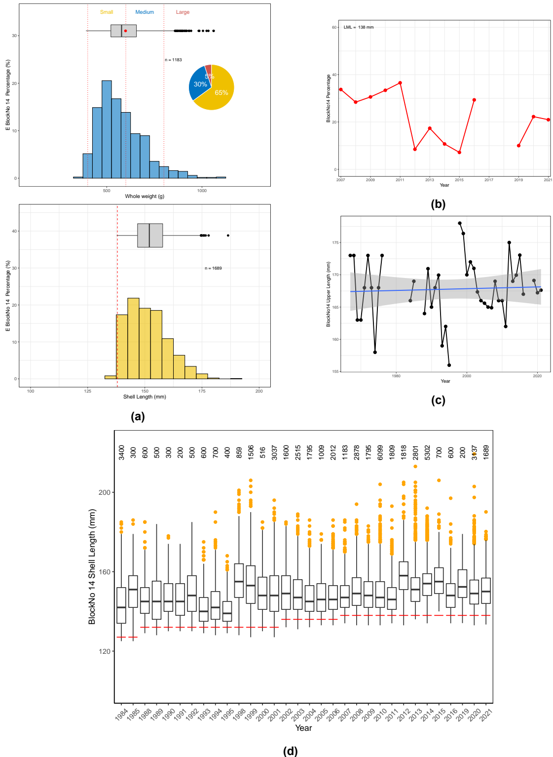
Figure 3.73: Block 14 EZ: a) Weight (top) and length (bottom) frequency distributions recorded at processing factories in 2021. Horizontal box plots represent summary weight and length distributions. Pie plot represents percentage composition of weight gradings (vertical dashed red lines) for abalone weighed; b) Proportion of commercial catch within 5 mm of current legal minimum length (LML); c) Upper 5th percentile of shell length frequency distributions; d) Boxplot of length frequency distributions between 1984 and 2021. Red line under each boxplot indicates LML for that year. Note: Red vertical dashed line represents a pause in sampling of more than one year prior to 2021. Number of abalone measured given above each boxplot.
