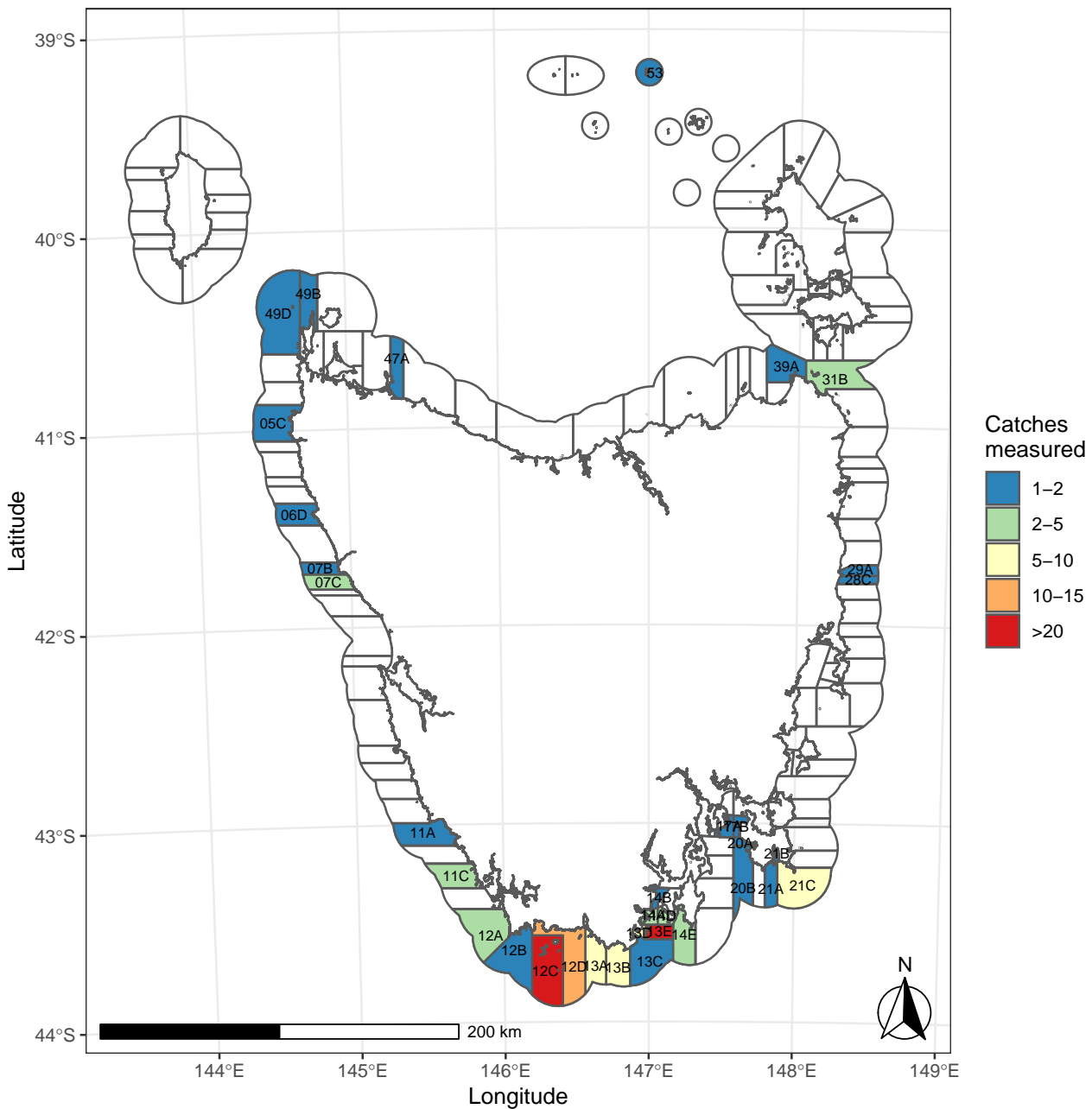
Figure 3.71: Distribution and number of commercial abalone catches sampled for length-frequency data across reporting Blocks during 2021.
