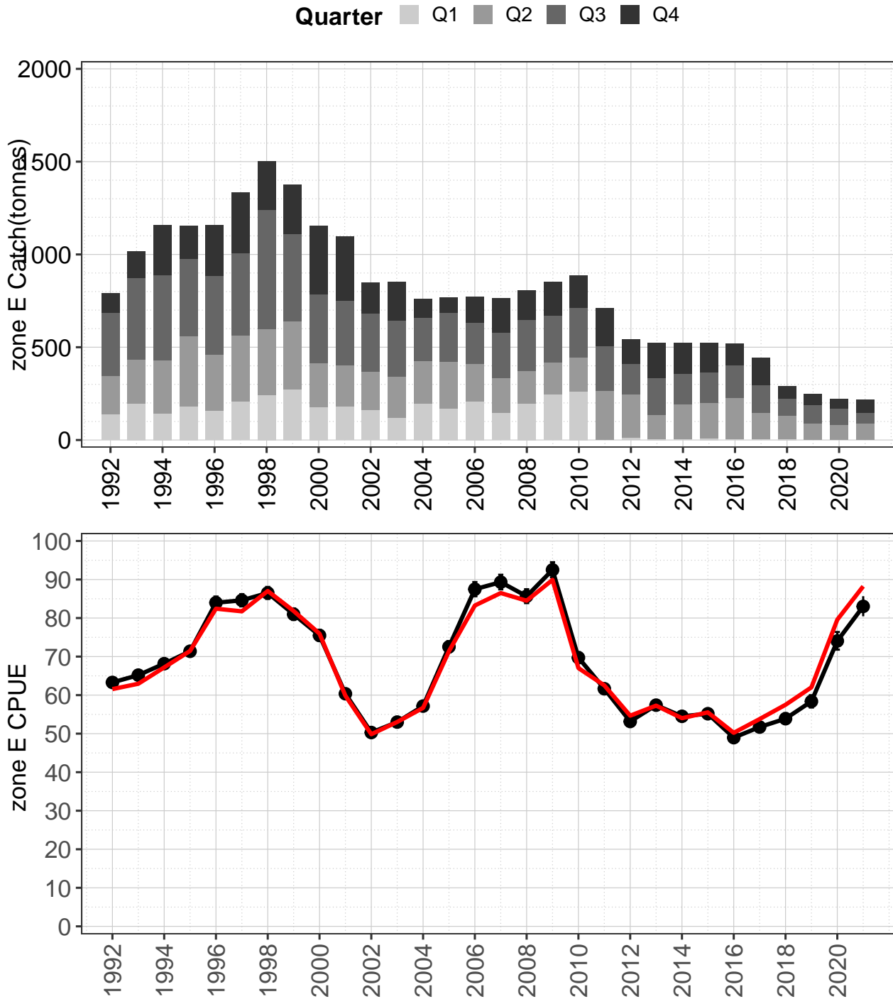
Figure 3.1: Zone-wide catch and catch rate for Eastern Zone blacklip abalone, 1992–2021. Upper plot: catch (t) by quarter pooled across blocks currently classified as Eastern Zone. Lower Plot: standardised CPUE (black line) and geometric mean CPUE (red line).
