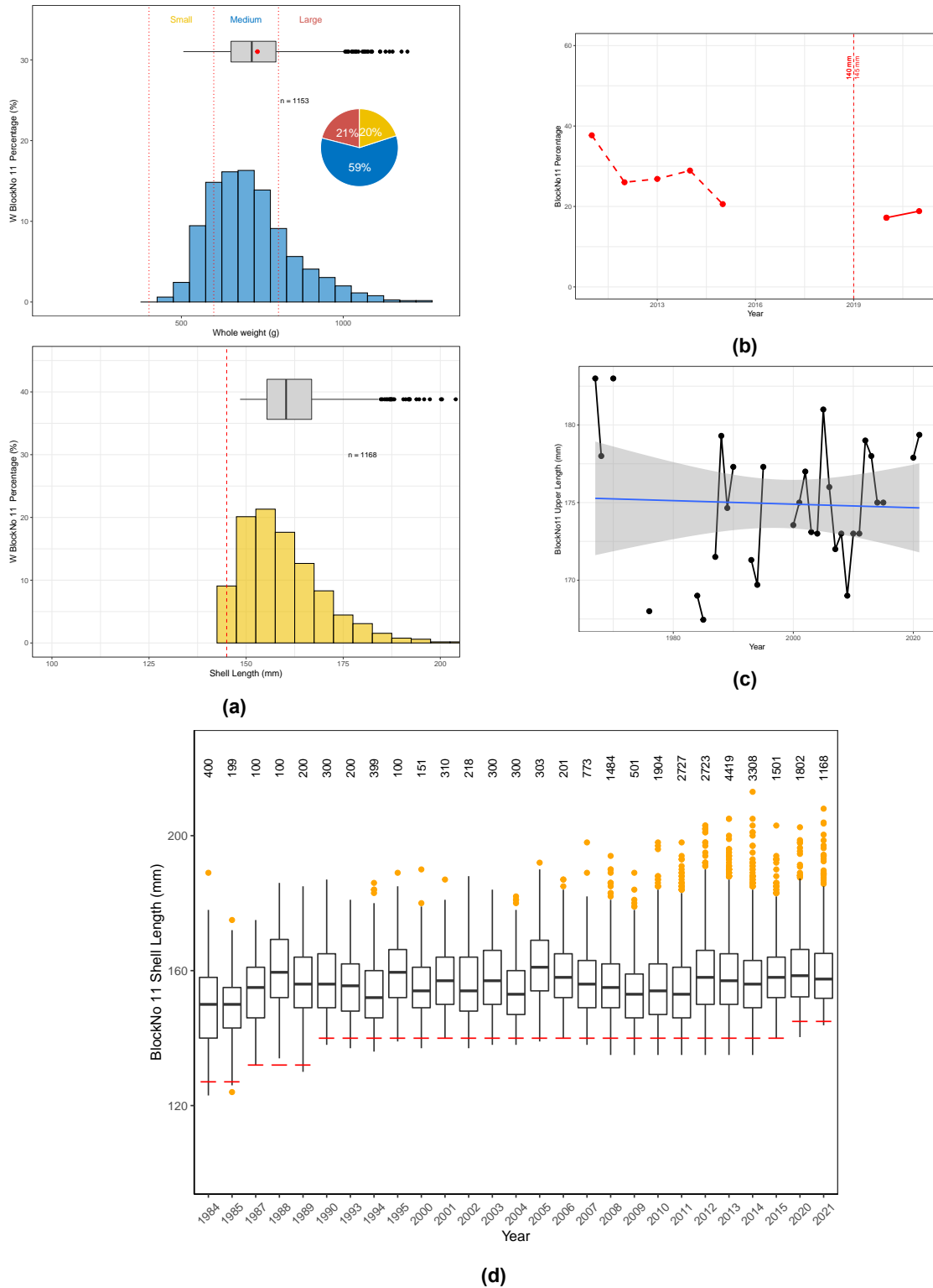
Figure 3.82: Block 11 WZ: a) Weight (top) and length (bottom) frequency distributions recorded at processing factories in 2021. Horizontal box plots represent summary weight and length distributions. Pie plot represents percentage composition of weight gradings (vertical dashed red lines) for abalone weighed; b) proportion of commercial catch within 5 mm of current legal minimum length (LML). Note: Dashed red line are catch proportions prior to LML change (vertical dashed red line) within 5 mm of current LML; c) Upper 5th percentile of shell length frequency distributions; d) Boxplot of length frequency distributions between 1984 and 2021. Red line under each boxplot indicates LML for that year. Note: Red vertical dashed line represents a pause in sampling of more than one year prior to 2021. Number of abalone measured given above each boxplot.
