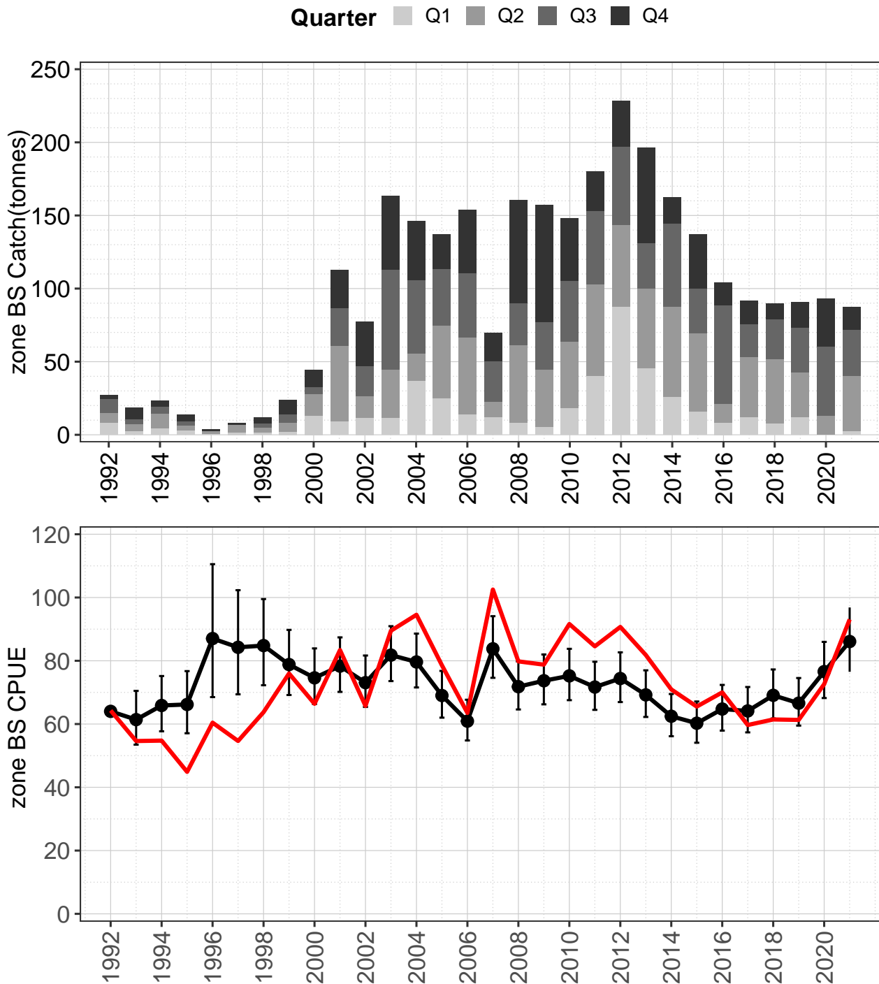
Figure 3.45: Zone-wide catch and catch rate for Bass Strait Zone blacklip abalone, 1992–2021. Upper plot: catch (t) by quarter pooled across blocks currently classified as Bass Strait Zone. Lower Plot: standardised CPUE (black line) and geometric mean CPUE (red line).
