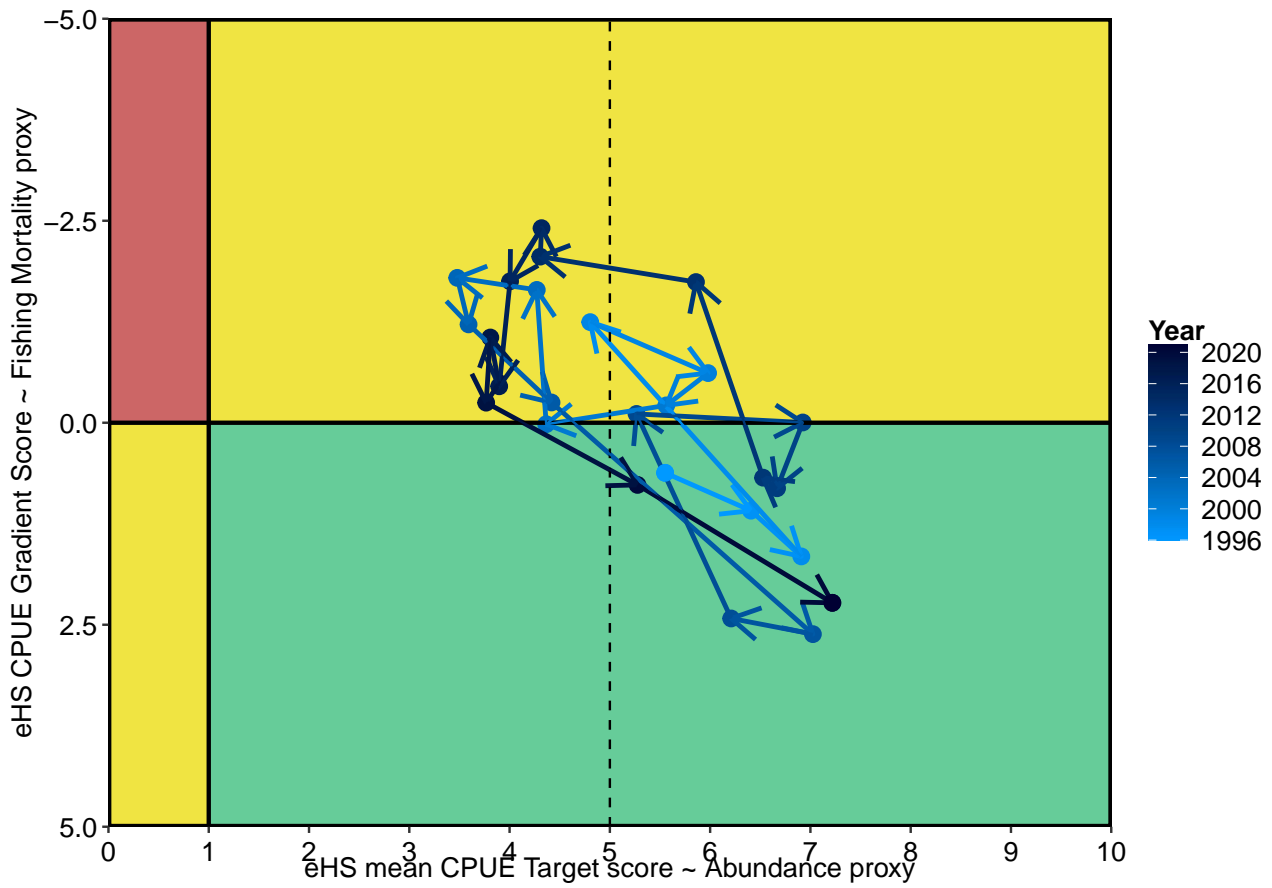
Figure 3.64: Phase plot of fishing mortality and abundance proxies for greenlip abalone, 1996–2021. The Gradient 4 PM (y-axis) is used as a proxy for fishing mortality, and the Target CPUE PM is used as a proxy for abundance. Zone score is calculated as a catch-weighted mean of individual regional scores.
