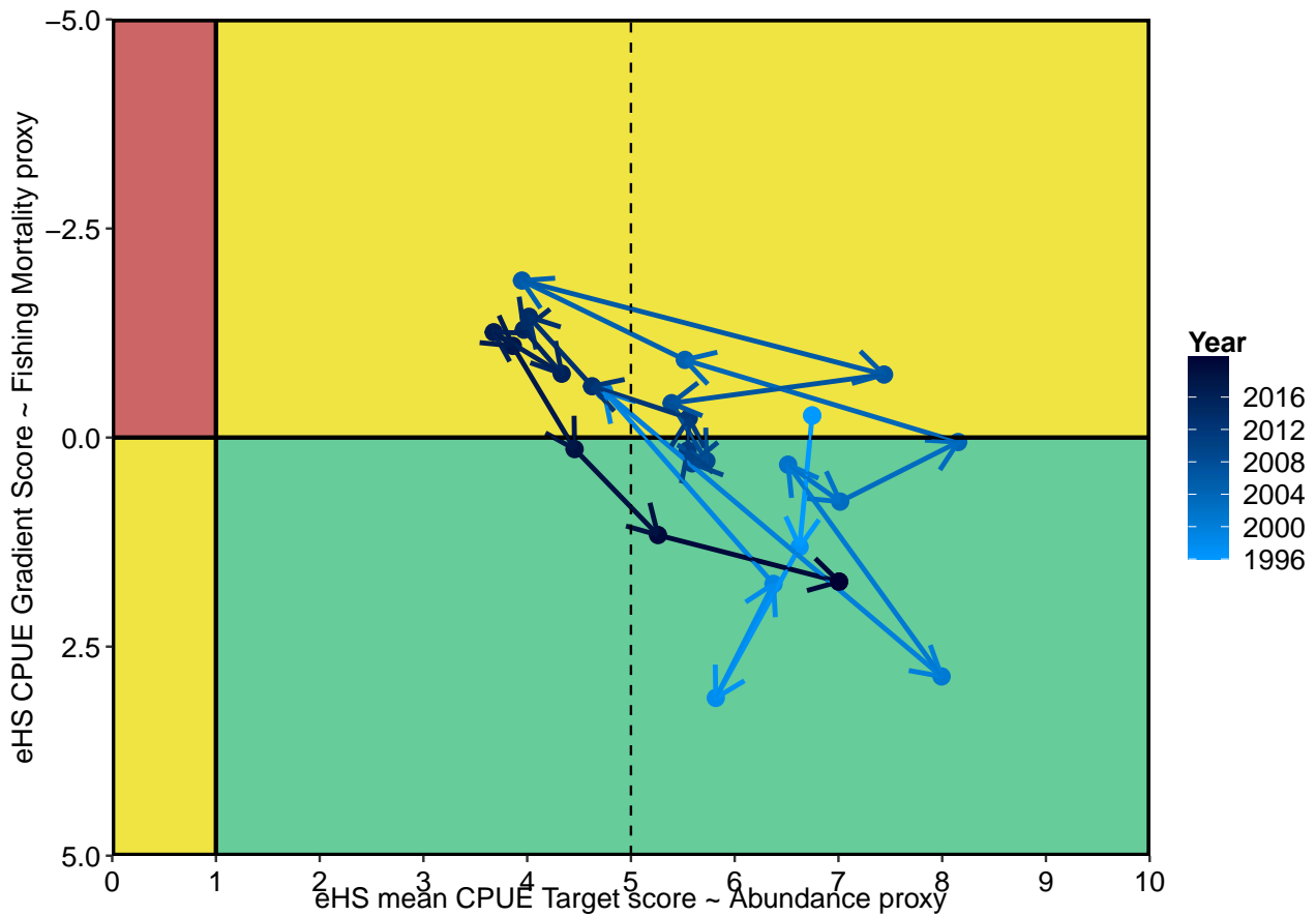
Figure 3.48: Phase plot of fishing mortality and abundance proxies for Bass Strait Zone blacklip abalone, 1996–2021. The Gradient 4 PM (y-axis) is used as a proxy for fishing mortality, and the Target CPUE PM is used as a proxy for abundance. Zone score is calculated as a catch-weighted mean of individual block scores.
