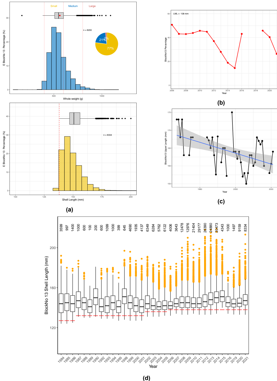
Figure 3.72: Block 13 EZ: a) Weight (top) and length (bottom) frequency distributions recorded at processing factories in 2021. Horizontal box plots represent summary weight and length distributions. Pie plot represents percentage composition of weight gradings (vertical dashed red lines) for abalone weighed; b) Proportion of commercial catch within 5 mm of current legal minimum length (LML); c) Upper 5th percentile of shell length frequency distributions; d) Boxplot of length frequency distributions between 1984 and 2021. Red line under each boxplot indicates LML for that year. Note: Red vertical dashed line represents a pause in sampling of more than one year prior to 2021. Number of abalone measured given above each boxplot.
