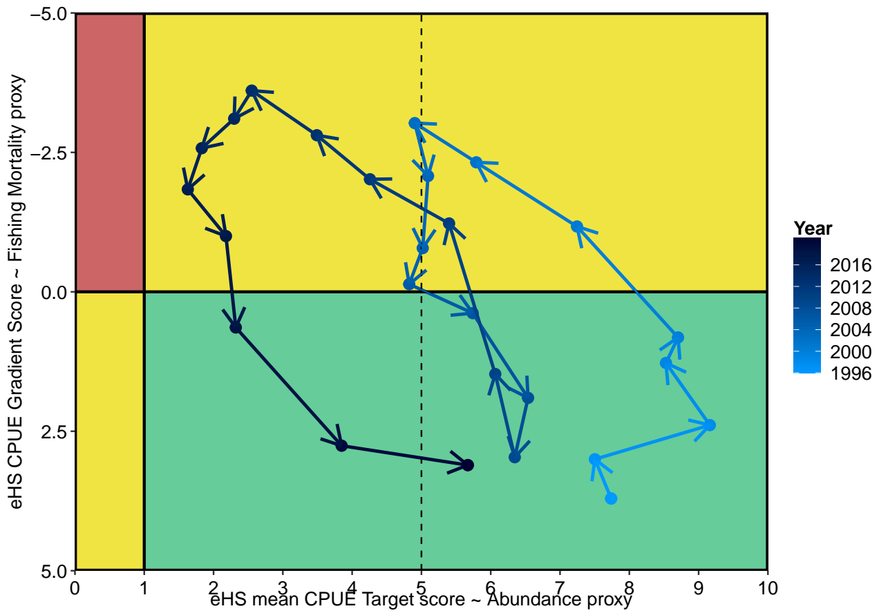
Figure 3.35: Phase plot of fishing mortality and abundance proxies for Northern Zone blacklip abalone, 1996–2021. The Gradient 4 PM (y-axis) is used as a proxy for fishing mortality, and the Target CPUE PM is used as a proxy for abundance. Zone score is calculated as a catch-weighted mean of individual block scores.
