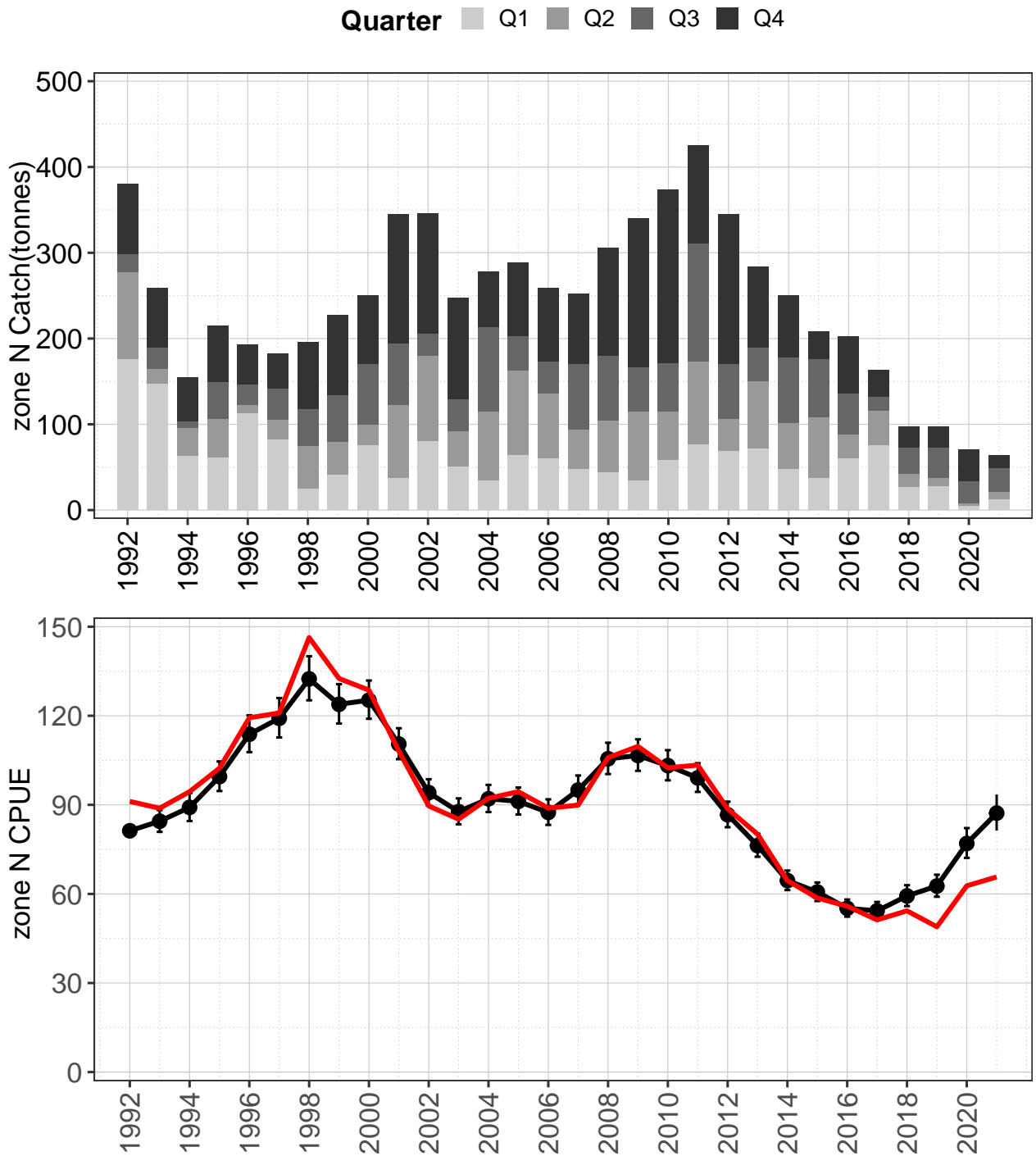
Figure 3.32: Zone-wide catch and catch rate for Northern Zone blacklip abalone, 1992–2021. Upper plot: catch (t) by quarter pooled across blocks currently classified as Northern Zone. Lower Plot: standardised CPUE (black line) and geometric mean CPUE (red line).
