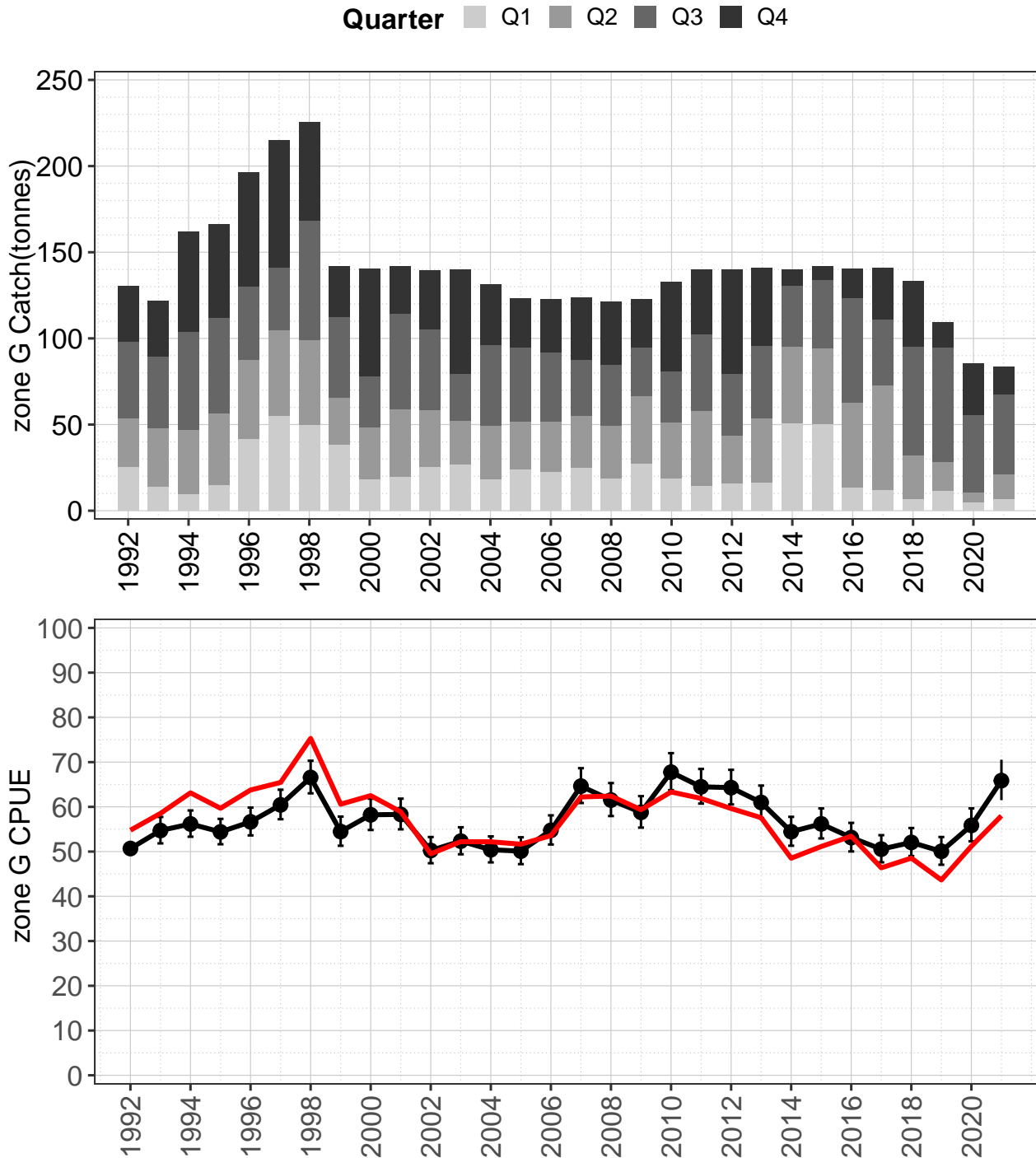
Figure 3.61: Zone-wide catch and catch rate for greenlip abalone, 1992–2021. Upper plot: catch (t) by quarter pooled across blocks. Lower Plot: standardised CPUE (black line) and geometric mean CPUE (red line).
