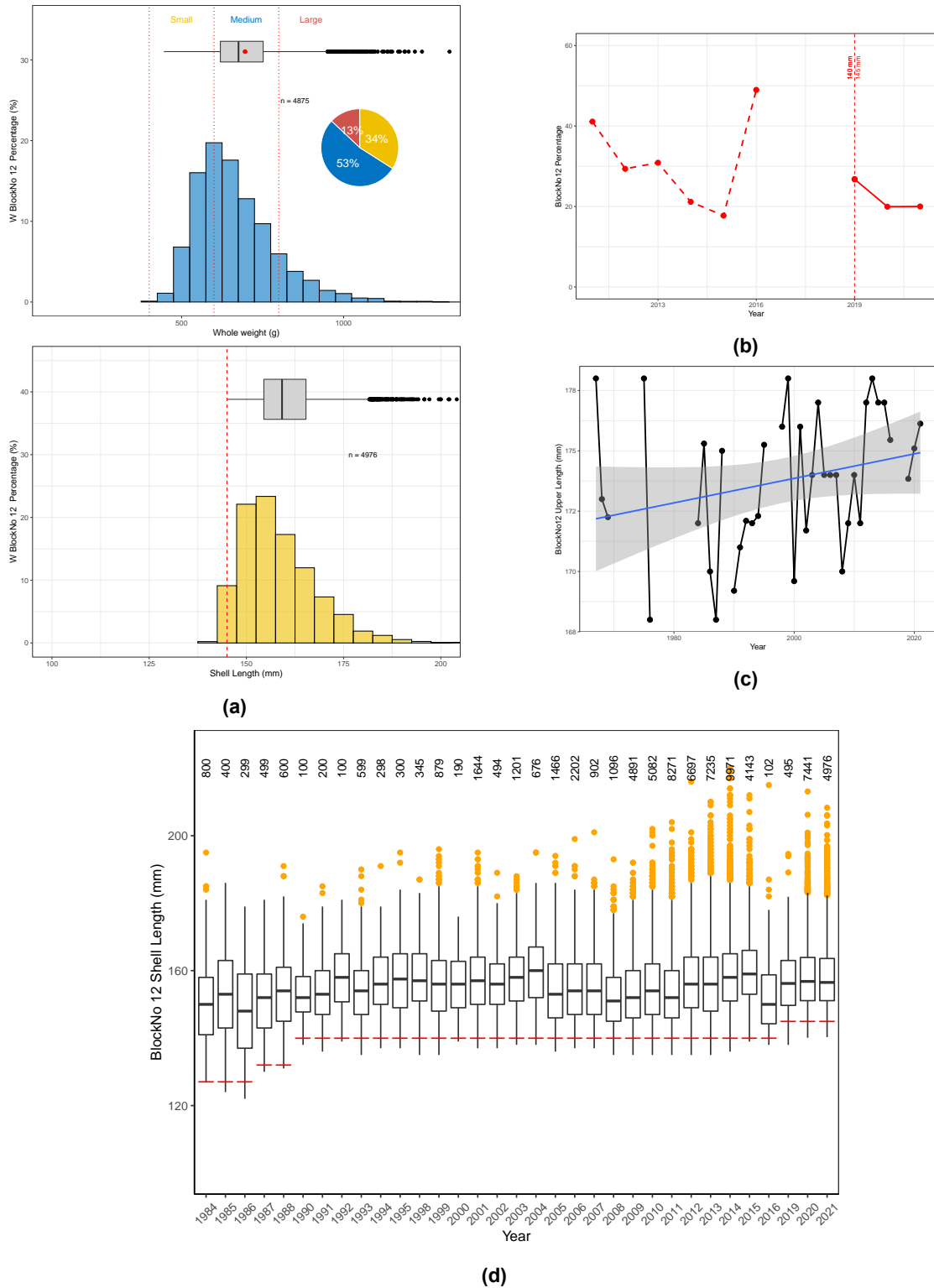
Figure 3.83: Block 12 WZ: a) Weight (top) and length (bottom) frequency distributions recorded at processing factories in 2021. Horizontal box plots represent summary weight and length distributions. Pie plot represents percentage composition of weight gradings (vertical dashed red lines) for abalone weighed; b) proportion of commercial catch within 5 mm of current legal minimum length (LML). Note: Dashed red line are catch proportions prior to LML change (vertical dashed red line) within 5 mm of current LML; c) Upper 5th percentile of shell length frequency distributions; d) Boxplot of length frequency distributions between 1984 and 2021. Red line under each boxplot indicates LML for that year. Note: Red vertical dashed line represents a pause in sampling of more than one year prior to 2021. Number of abalone measured given above each boxplot.
