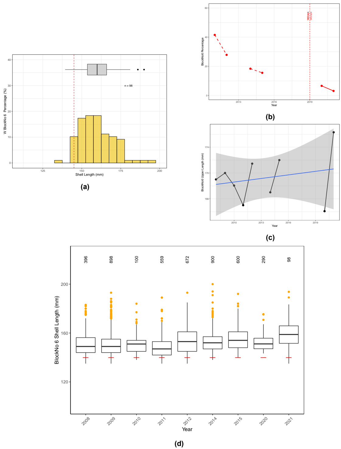
Figure 3.79: Block 6 WZ: a) Length frequency distribution recorded by diver-based measuring board in 2021. Horizontal box plots represent summary length distribution. Vertical dashed red line represents LML; b) Proportion of commercial catch within 5 mm of current legal minimum length (LML); c) Upper 5th percentile of shell length frequency distributions; d) Boxplot of length frequency distributions between 1984 and 2021. Red line under each boxplot indicates LML for that year. Note: Red vertical dashed line represents a pause in sampling of more than one year prior to 2021. Number of abalone measured given above each boxplot.
