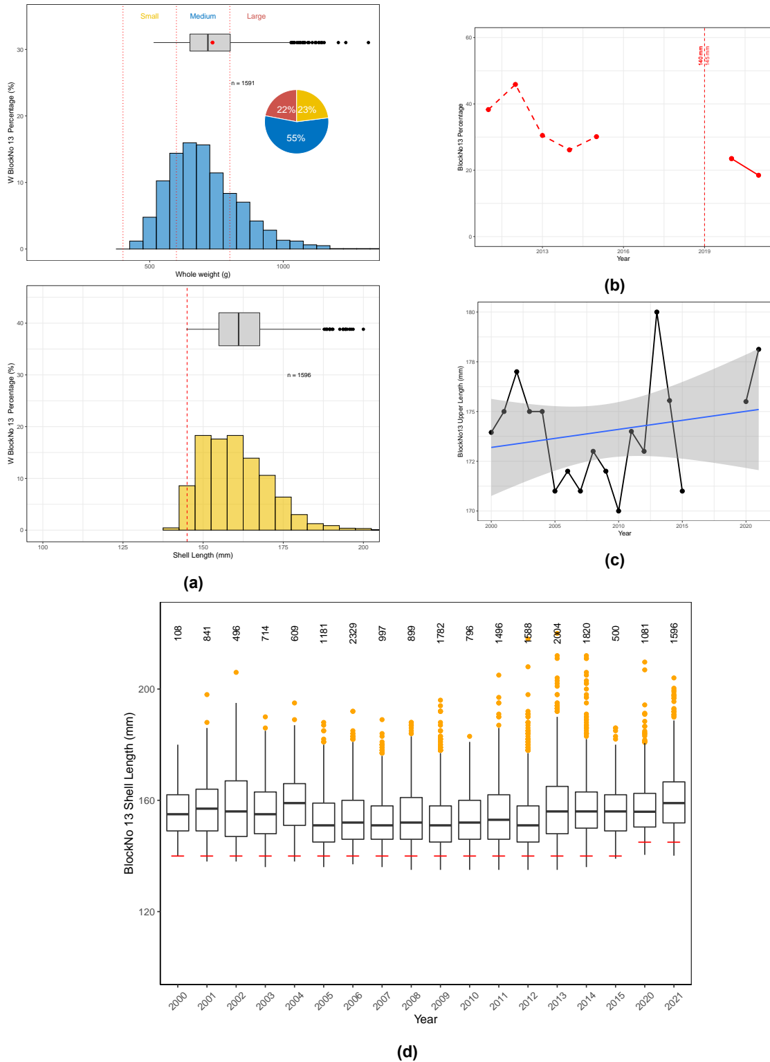
Figure 3.84: Block 13 WZ: a) Weight (top) and length (bottom) frequency distributions recorded at processing factories in 2021. Horizontal box plots represent summary weight and length distributions. Pie plot represents percentage composition of weight gradings (vertical dashed red lines) for abalone weighed; b) proportion of commercial catch within 5 mm of current legal minimum length (LML). Note: Dashed red line are catch proportions prior to LML change (vertical dashed red line) within 5 mm of current LML; c) Upper 5th percentile of shell length frequency distributions; d) Boxplot of length frequency distributions between 1984 and 2021. Red line under each boxplot indicates LML for that year. Note: Red vertical dashed line represents a pause in sampling of more than one year prior to 2021. Number of abalone measured given above each boxplot.
