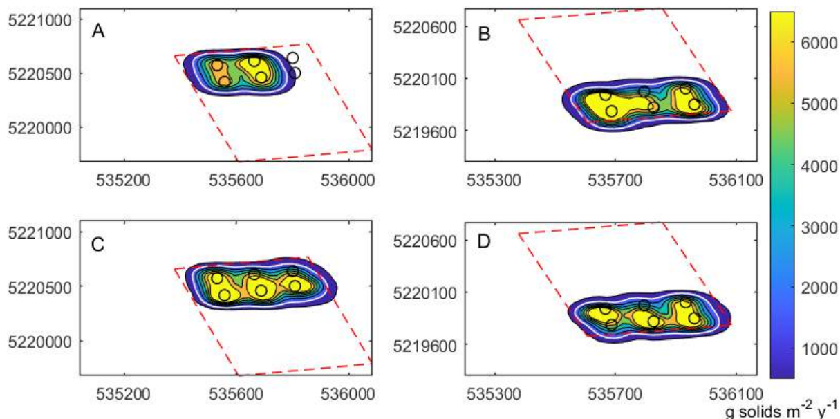
Figure 7.2-9 Deposition rates (g solids m -2 y -1 ) at Storm Bay 1 as predicted by NewDEPOMOD. A represents deposition around northern cage grid for January 2017, B is southern grid January 2017, C is northern grid June 2017, D is southern grid for June 2017. The 1500 g solids m -2 y -1 is applied in each Figure as an expected benthic impact threshold (white line). The black circles are cages, whilst the red dashed line represents the lease boundary.
