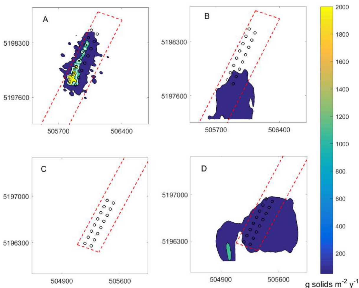
Figure 7.2-11 Deposition rates ( \text{g solids m}^{-2} \text{ y}^{-1} ) at East of Lippies based on feed rates in Table 7.2-2. A is DEPOMOD result for northern grid in January 2018, B is NewDEPOMOD results northern grid in January 2018, C is DEPOMOD results for southern grid in November 2017, and D the NewDEPOMOD result southern grid in November 2017. The white line (visible only in A) is the 1500 ( \text{g solids m}^{-2} \text{ y}^{-1} ) contour, or the expected benthic impact threshold. Black circles represent cages and the red dashed lines represent the lease boundary.
